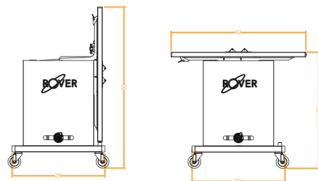
SIDE VIEWS
