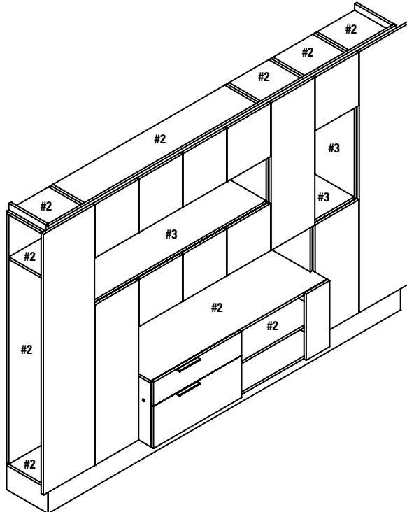
Isometric View
