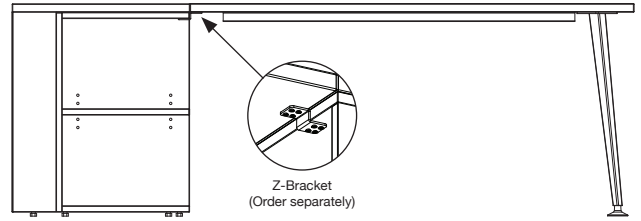
Standard Run-Off Connection (Desk Shell and Floor Bookcase with Run-Off) Desk Shell with Flushed Modesty and 18" Deep Floor Bookcase Shown
